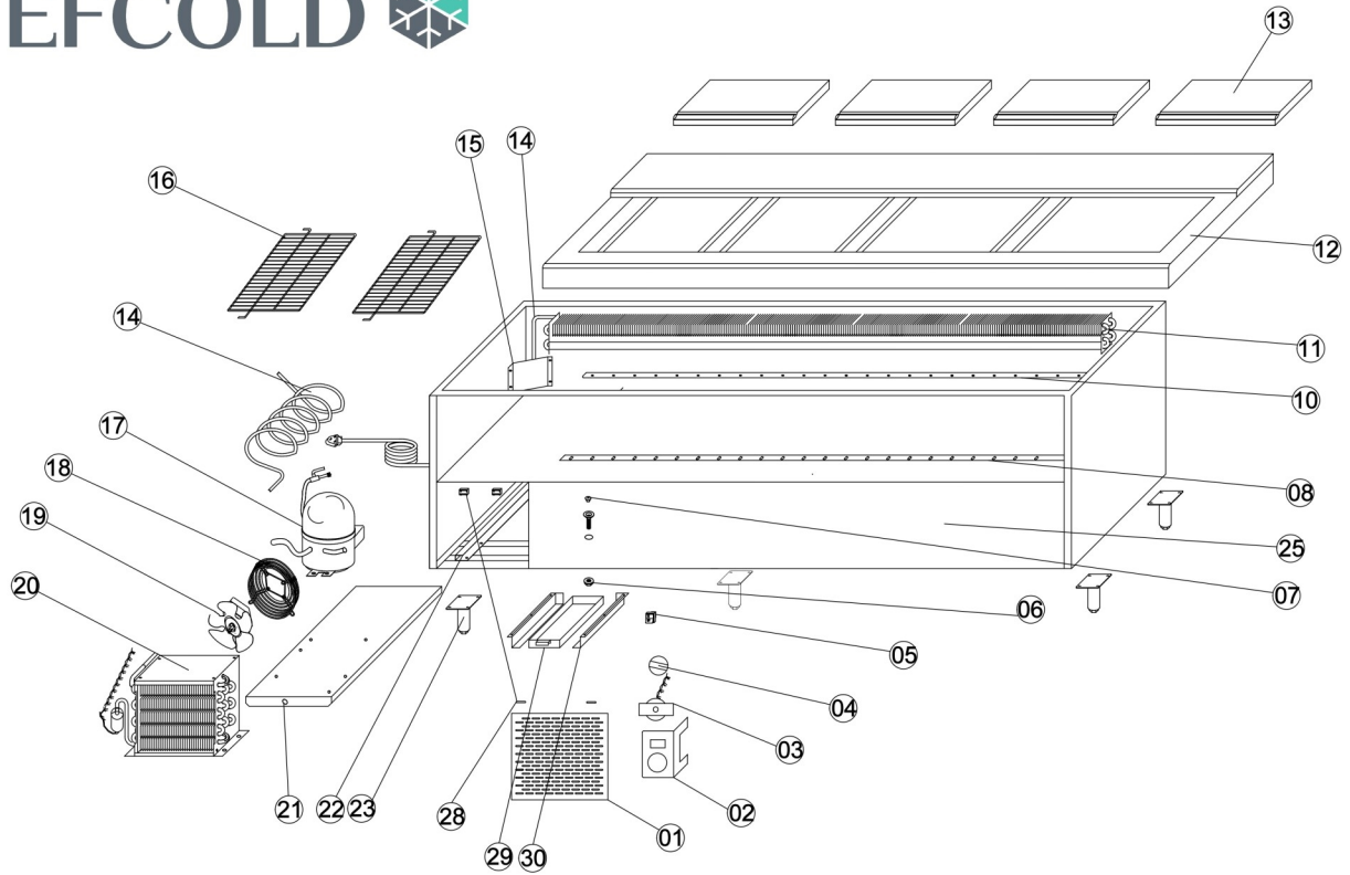
EXPLODED VIEW OF BHC250X1
