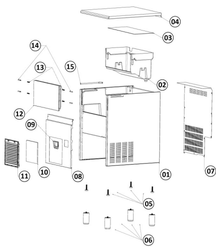
CABINET SYSTEM
