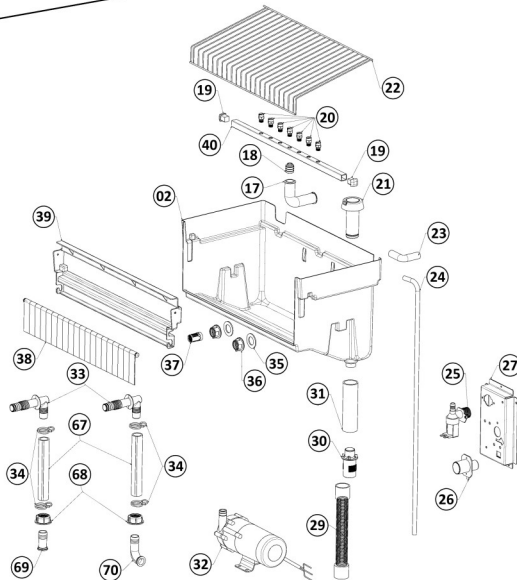
WATER DISTRIBUTION
