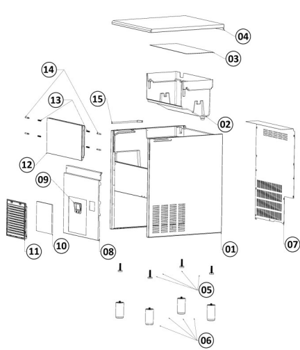
CABINET SYSTEM
